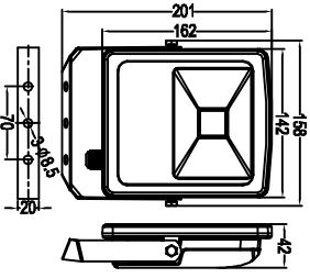
ZY-2085-20W COB
