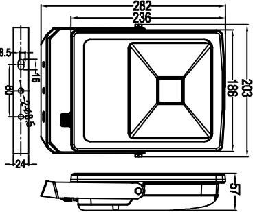
ZY-2085-50W COB
