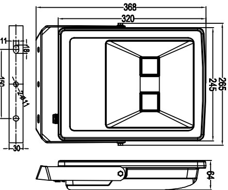
ZY-2085-100W COB
