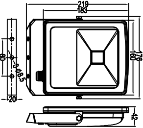
ZY-2085-30W COB
