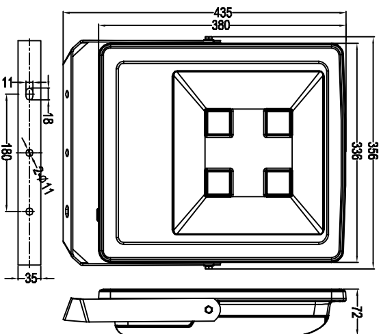
ZY-2085-200W COB
