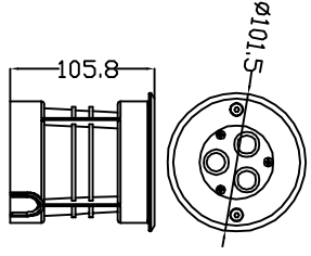
LED 3W
