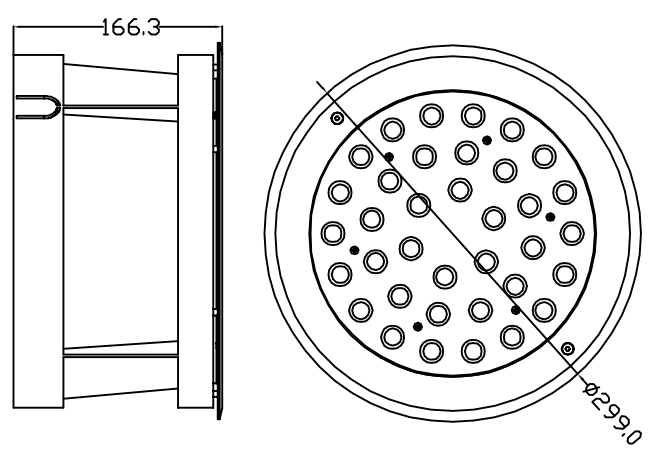
LED 36W
