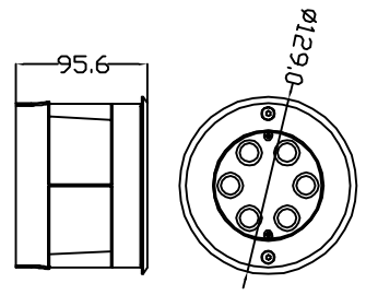
LED 6W
