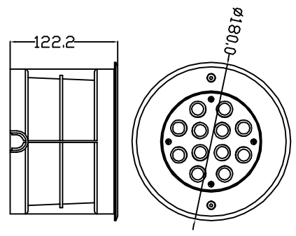
LED 9W/12W
